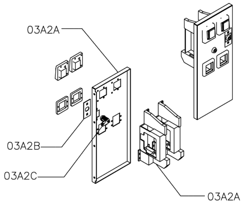
03A2. CAR A002A2 DOUBLE COIN ASSEMBLY
